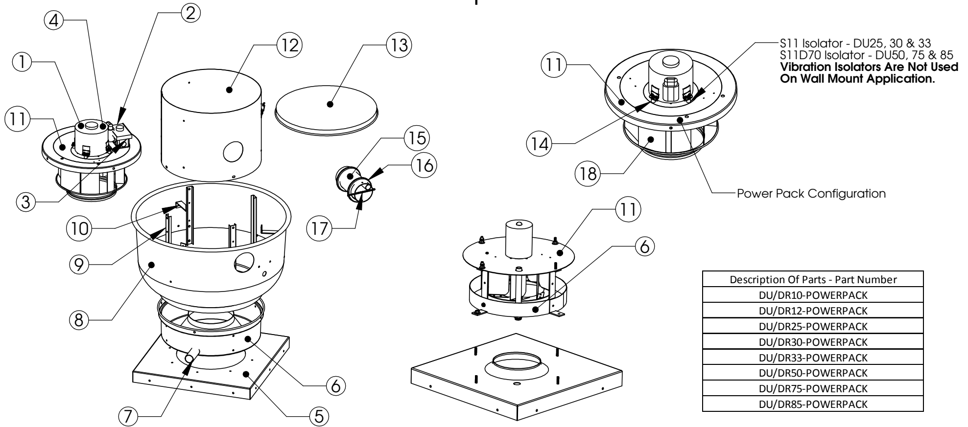
Direct Drive - Motor - Part Information.
